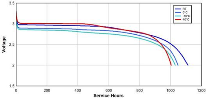
Temperature Discharge 30K Ohm Continuous to 2.0V
